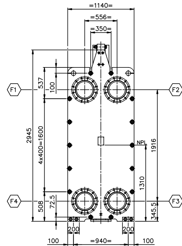
VIEW P FRONT SIDE SCALE: 1/20
