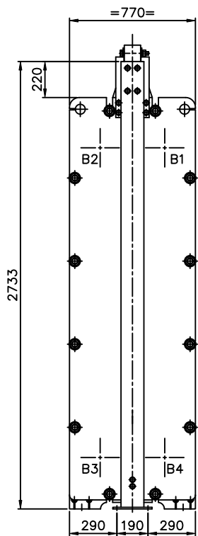
VIEW Q REAR SIDE SCALE: 1/15
