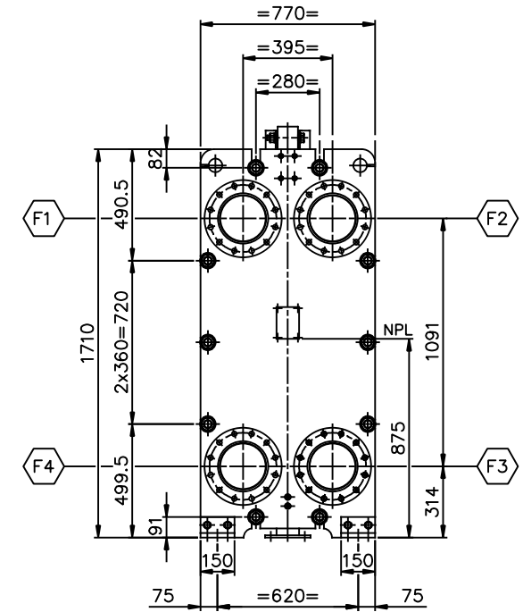
VIEW P FRONT SIDE SCALE: 1/15
