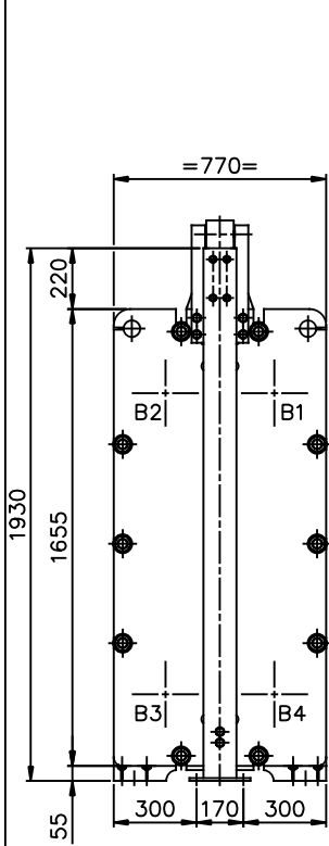
VIEW Q REAR SIDE SCALE: 1/15
