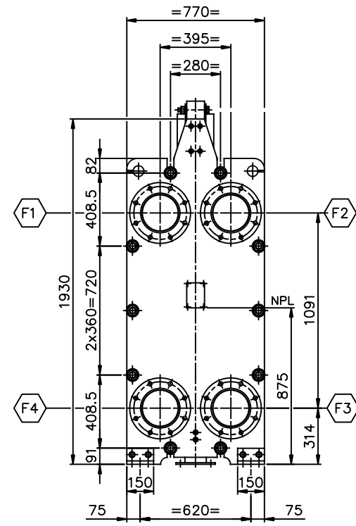
VIEW P FRONT SIDE SCALE: 1/15
