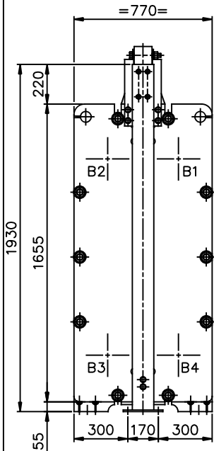
VIEW Q REAR SIDE SCALE: 1/15
