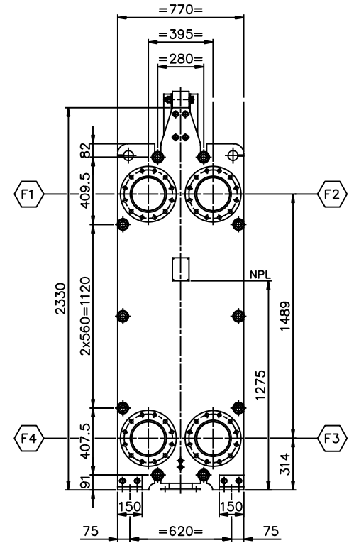
VIEW P FRONT SIDE SCALE: 1/15
