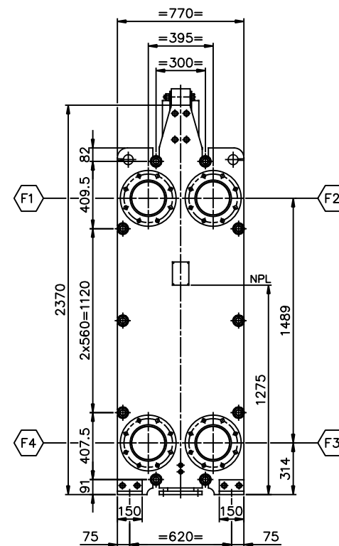
VIEW P FRONT SIDE SCALE: 1/15
