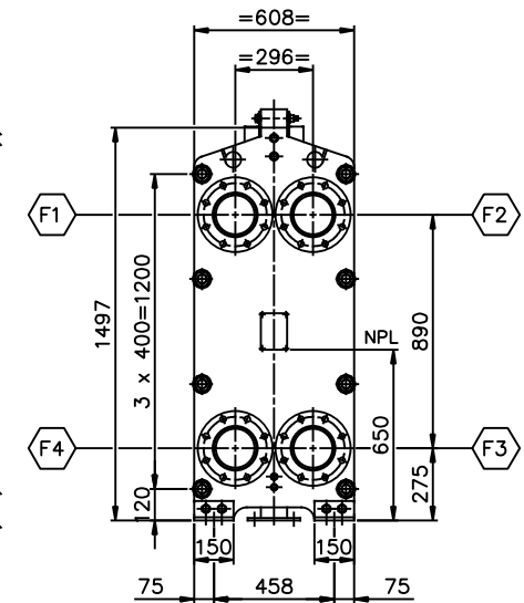
VIEW P FRONT SIDE SCALE: 1/15
