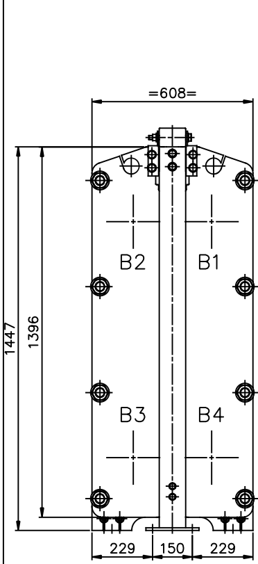
VIEW Q \Delta REAR SIDE SCALE: 1/10
