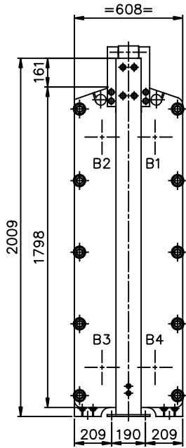
VIEW Q REAR SIDE SCALE: 1/15
