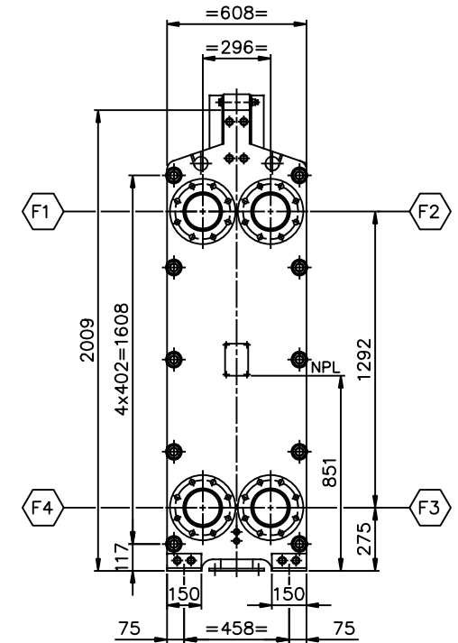
VIEW P FRONT SIDE SCALE: 1/15
