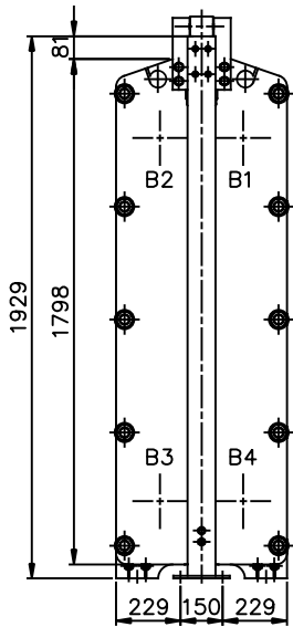
VIEW Q REAR SIDE SCALE: 1/15
