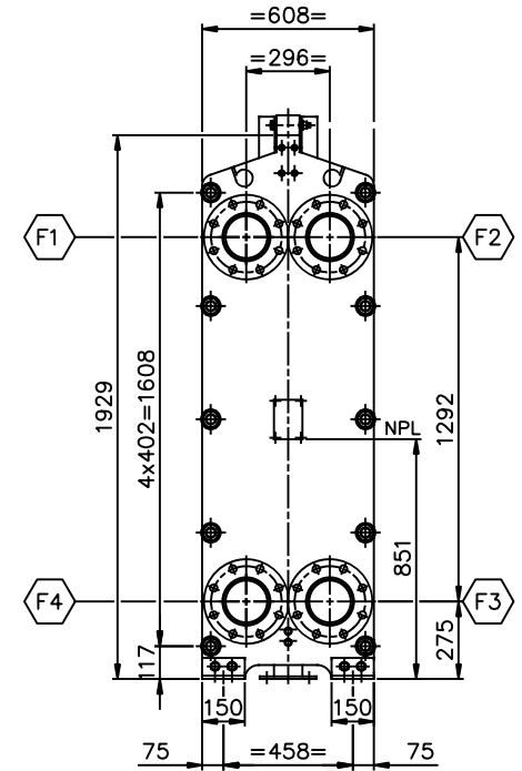
VIEW P FRONT SIDE SCALE: 1/15
