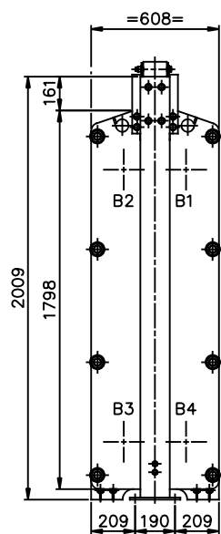
VIEW Q REAR SIDE SCALE: 1/15
