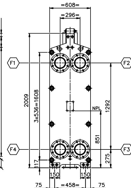
VIEW P FRONT SIDE SCALE: 1/15
