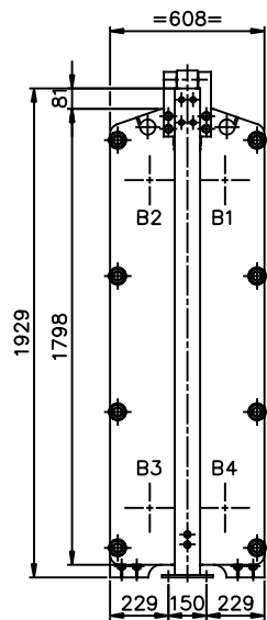
VIEW Q REAR SIDE SCALE: 1/15
