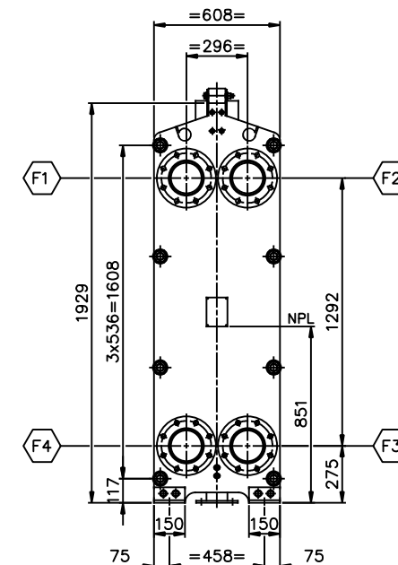
VIEW P \Delta FRONT SIDE SCALE: 1/15
