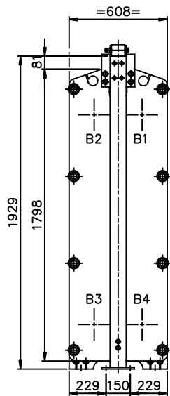
VIEW Q \Delta REAR SIDE SCALE: 1/15
