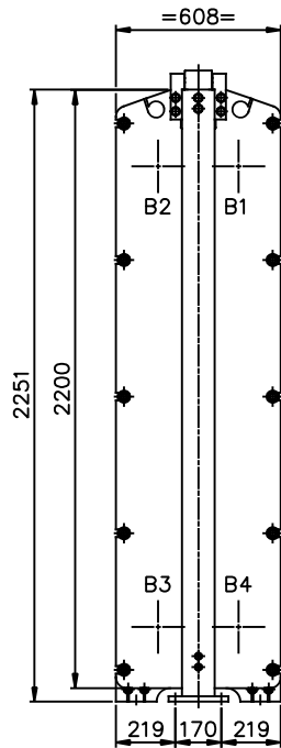
VIEW Q REAR SIDE SCALE: 1/15
