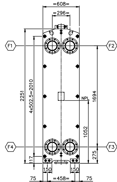
VIEW P FRONT SIDE SCALE: 1/15
