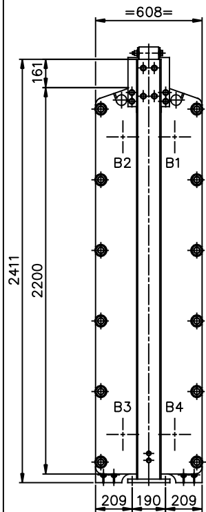
VIEW Q REAR SIDE SCALE: 1/15
