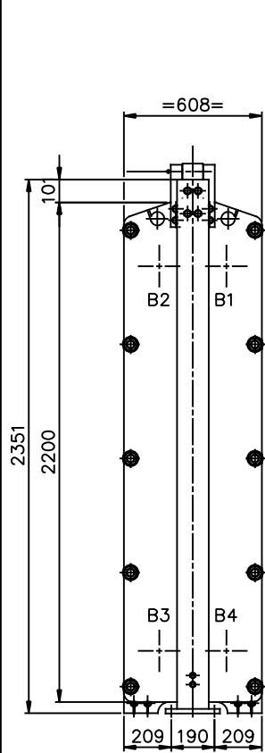
VIEW Q REAR SIDE SCALE: 1/15
