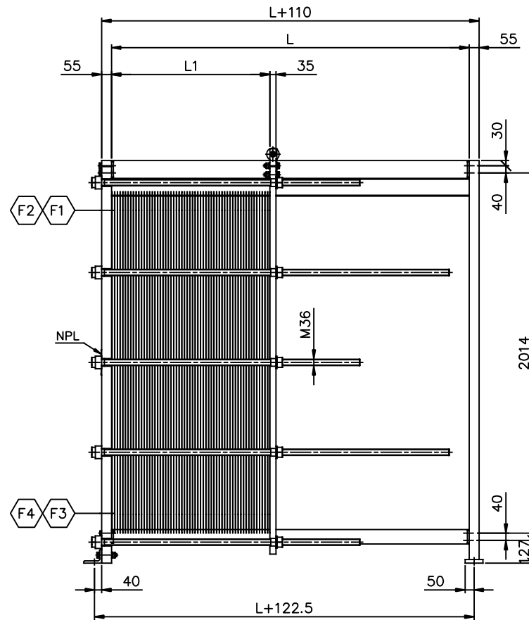
ELEVATION \triangle SCALE: 1/15
