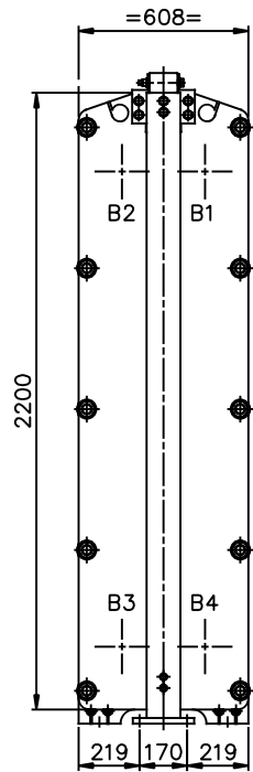
VIEW Q \triangle REAR SIDE SCALE: 1/15
