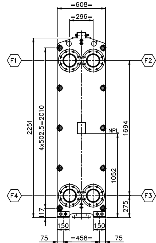
VIEW P \triangle FRONT SIDE SCALE: 1/15
