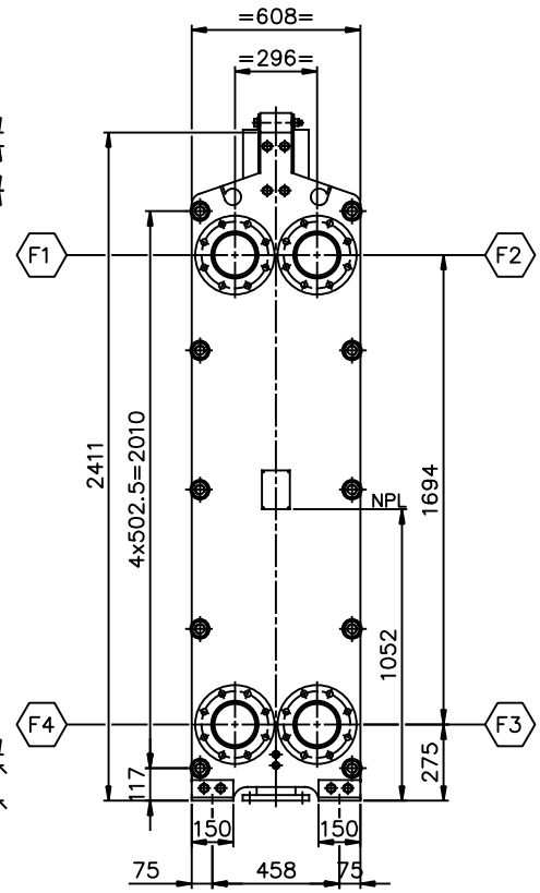
VIEW P FRONT SIDE SCALE: 1/15
