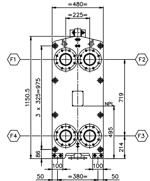
VIEW P FRONT SIDE SCALE: 1/10
