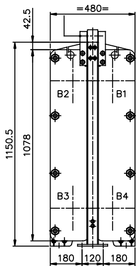
VIEW Q REAR SIDE SCALE: 1/10
