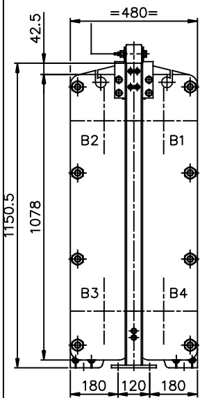
VIEW Q REAR SIDE SCALE: 1/10
