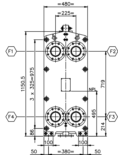
VIEW P FRONT SIDE SCALE: 1/10
