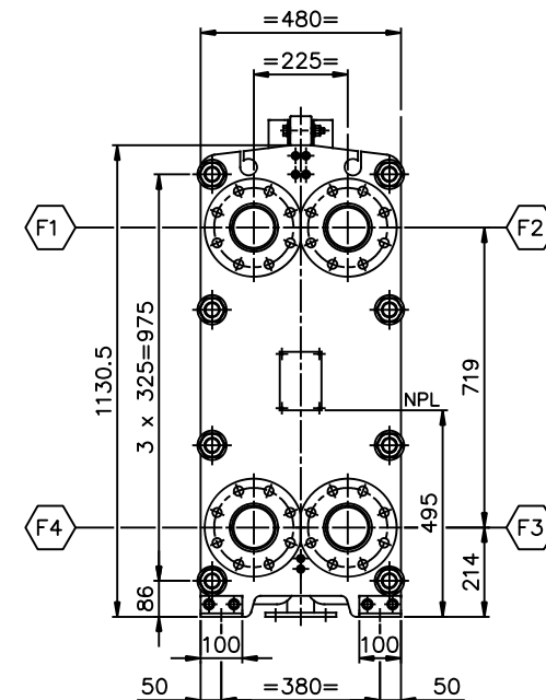
VIEW P FRONT SIDE SCALE: 1/10
