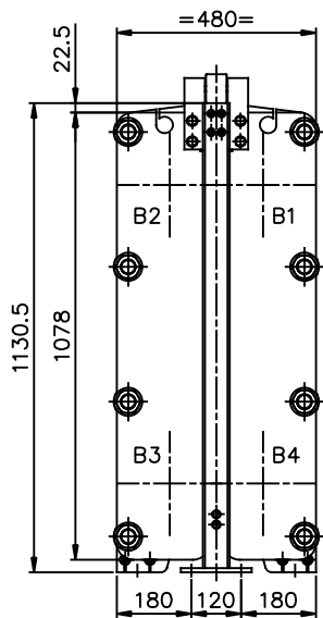
VIEW Q REAR SIDE SCALE: 1/10
