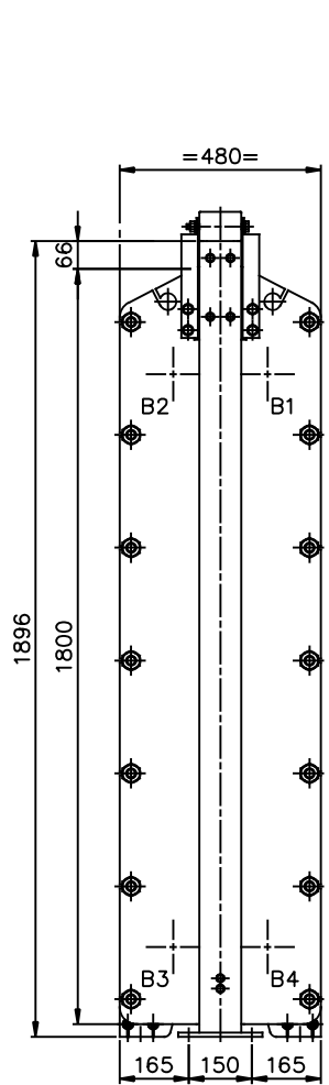
VIEW Q REAR SIDE SCALE: 1/10
