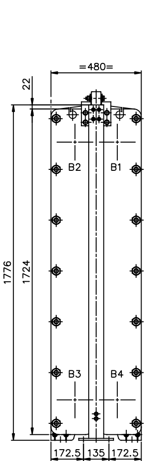
VIEW Q REAR SIDE SCALE: 1/10
