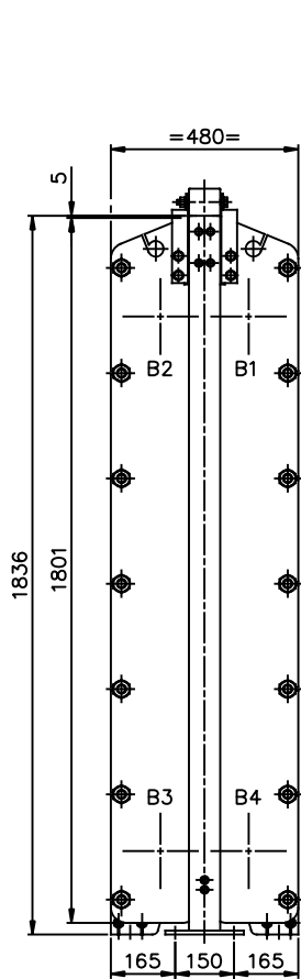
VIEW Q REAR SIDE SCALE: 1/10
