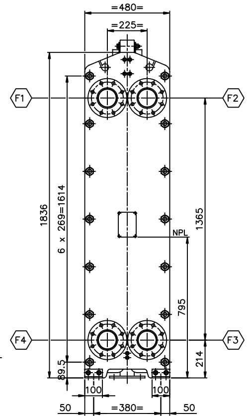
VIEW P FRONT SIDE SCALE: 1/10
