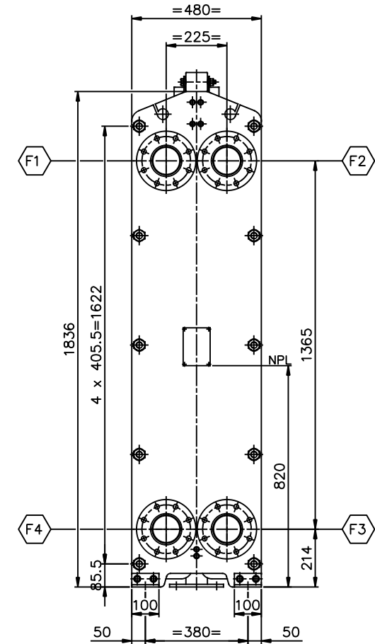
VIEW P FRONT SIDE SCALE: 1/10
