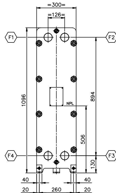
VIEW P FRONT SIDE SCALE: 1/7.5
