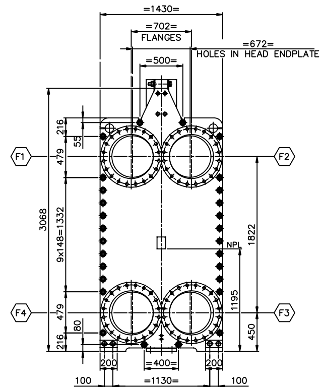
VIEW P FRONT SIDE SCALE: 1/20
