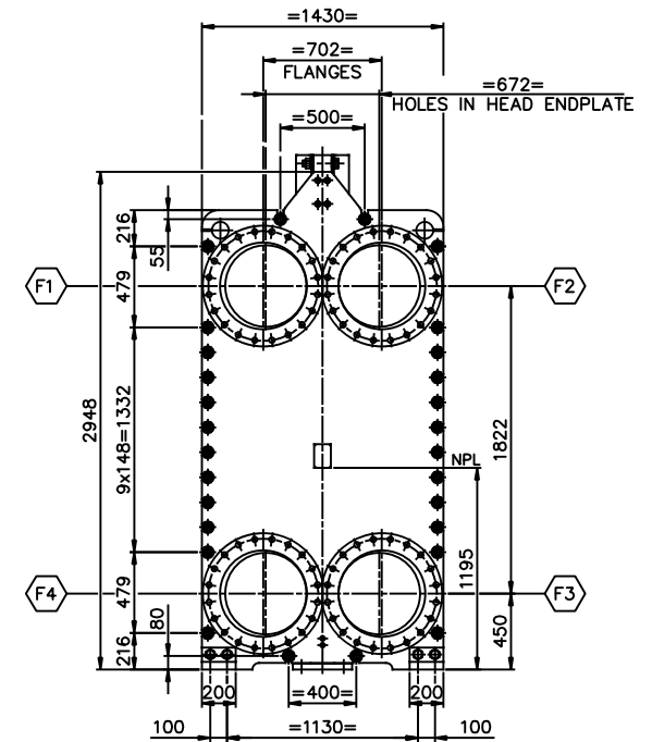
VIEW P FRONT SIDE SCALE: 1/20
