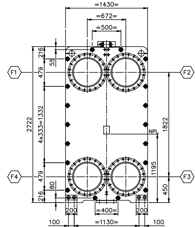
VIEW P FRONT SIDE SCALE: 1/20
