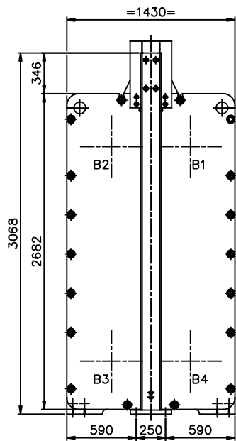
VIEW Q REAR SIDE SCALE: 1/20
