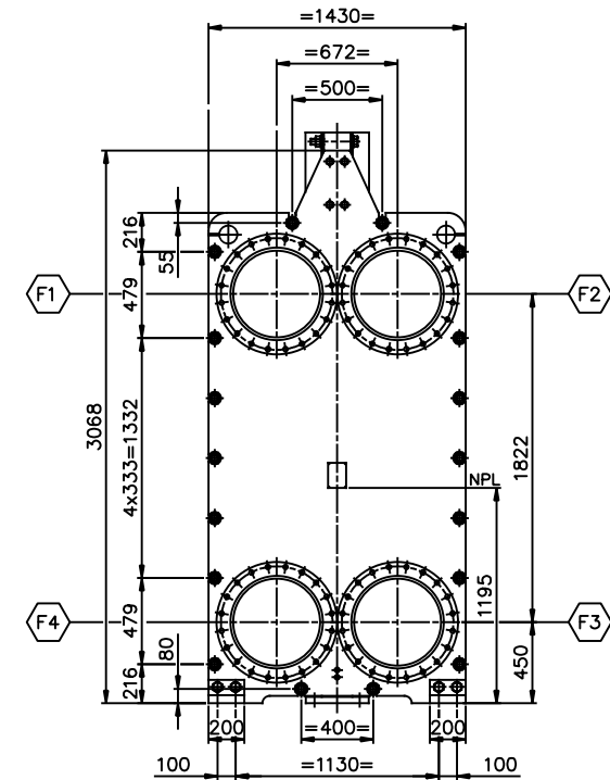
VIEW P FRONT SIDE SCALE: 1/20
