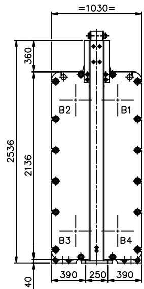
VIEW Q REAR SIDE SCALE: 1/20
