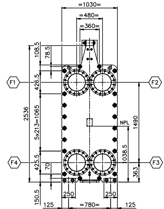
VIEW P FRONT SIDE SCALE: 1/20
