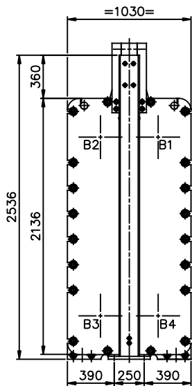
VIEW Q REAR SIDE SCALE: 1/20
