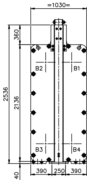
VIEW Q REAR SIDE SCALE: 1/20
