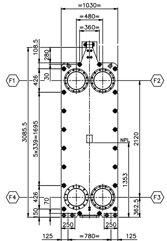
VIEW P FRONT SIDE SCALE: 1/20
