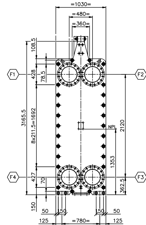
VIEW P FRONT SIDE SCALE: 1/20
