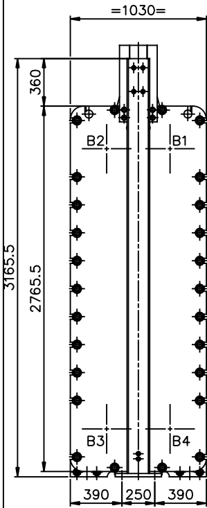
VIEW Q REAR SIDE SCALE: 1/20
