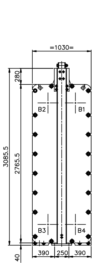
VIEW Q REAR SIDE SCALE: 1/20
